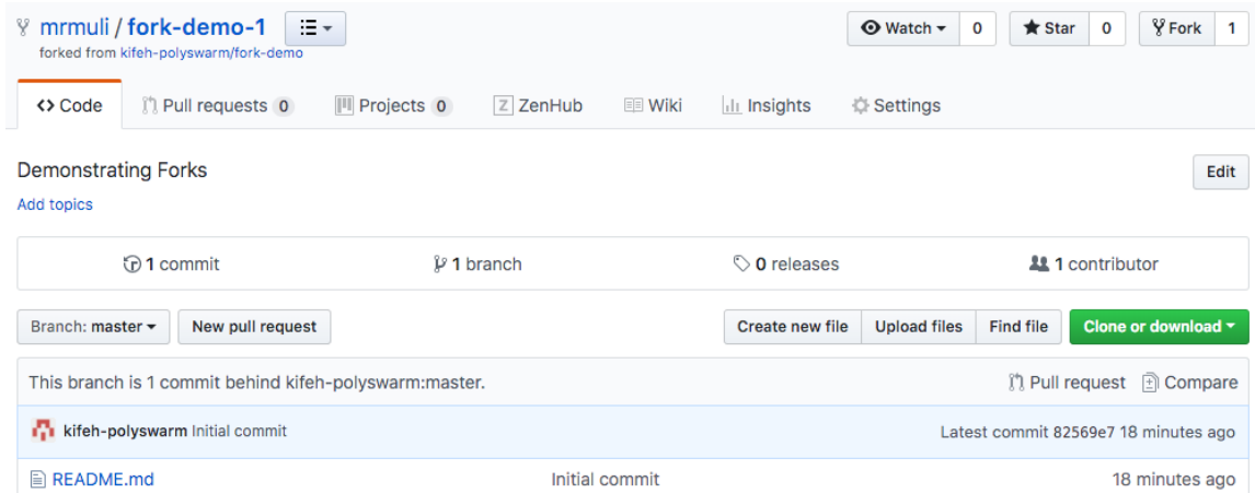
Figure 5.8: Using fork-demo-1
