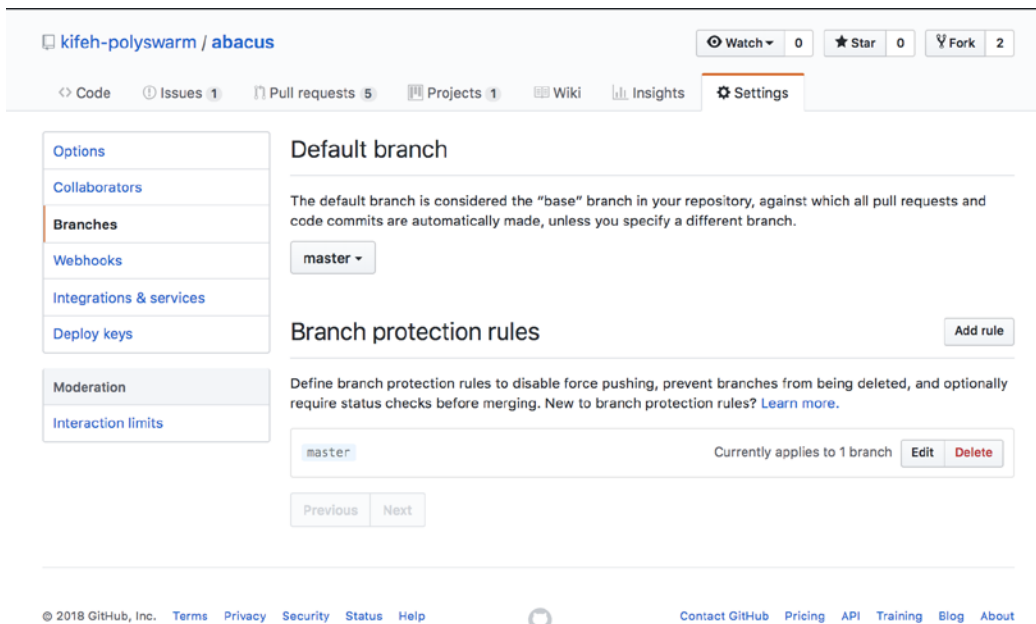
Figure 3.52: Branch rules
