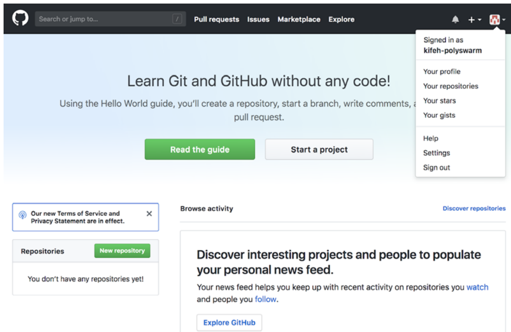
Figure 1.6: Account configuration
