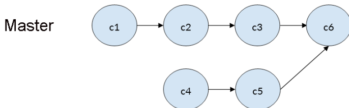
Figure 4.51: Merge Commit
