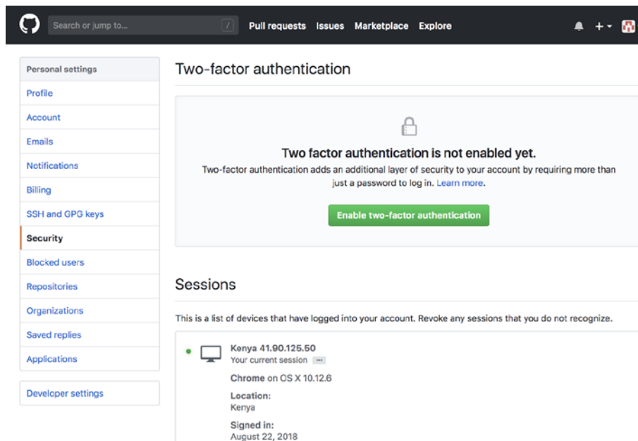
Figure 1.8: Two-factor authentication
