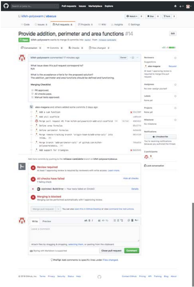
Figure 4.60: Providing functions
