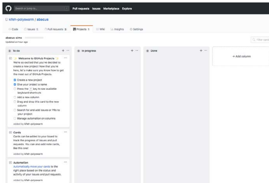
Figure 4.8: Adding cards
