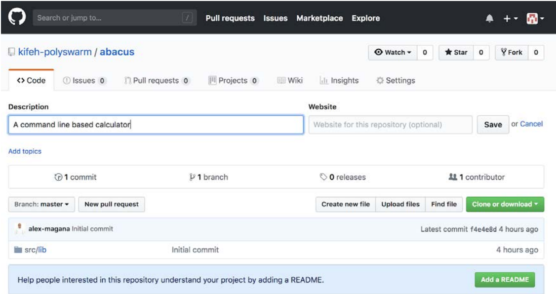
Figure 1.60: Description entry
