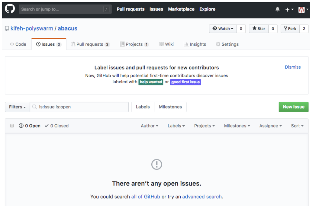
Figure 4.5: New issue
