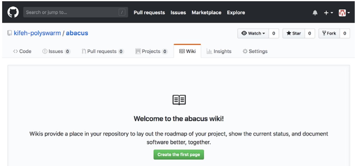
Figure 1.65: Abacus wiki
