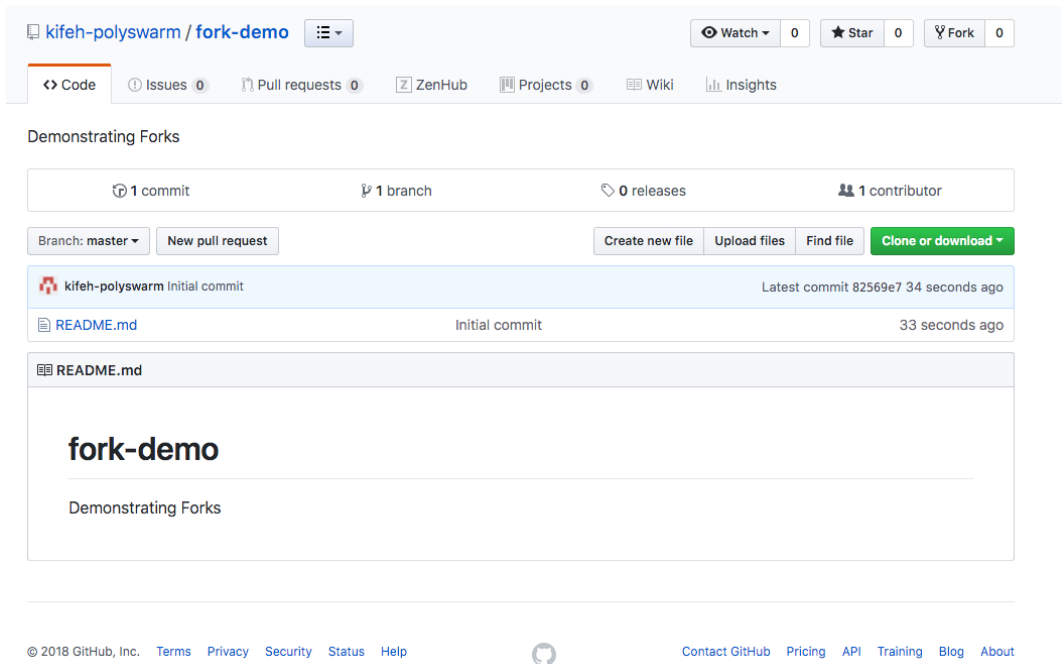
Figure 5.2: Fork demo
