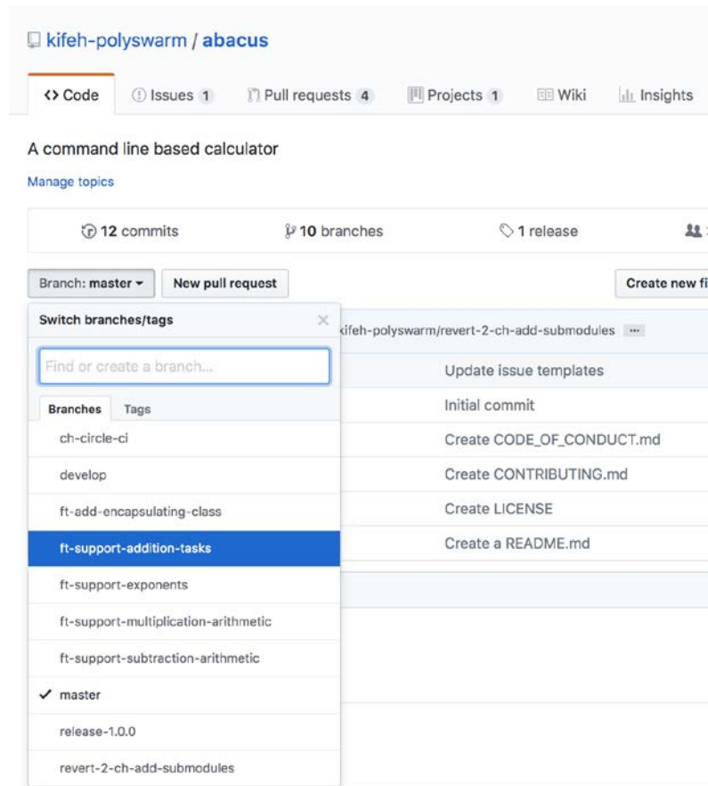
Figure 4.19: Branch selector
