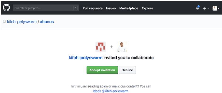
Figure 1.54: Accepting invitation
