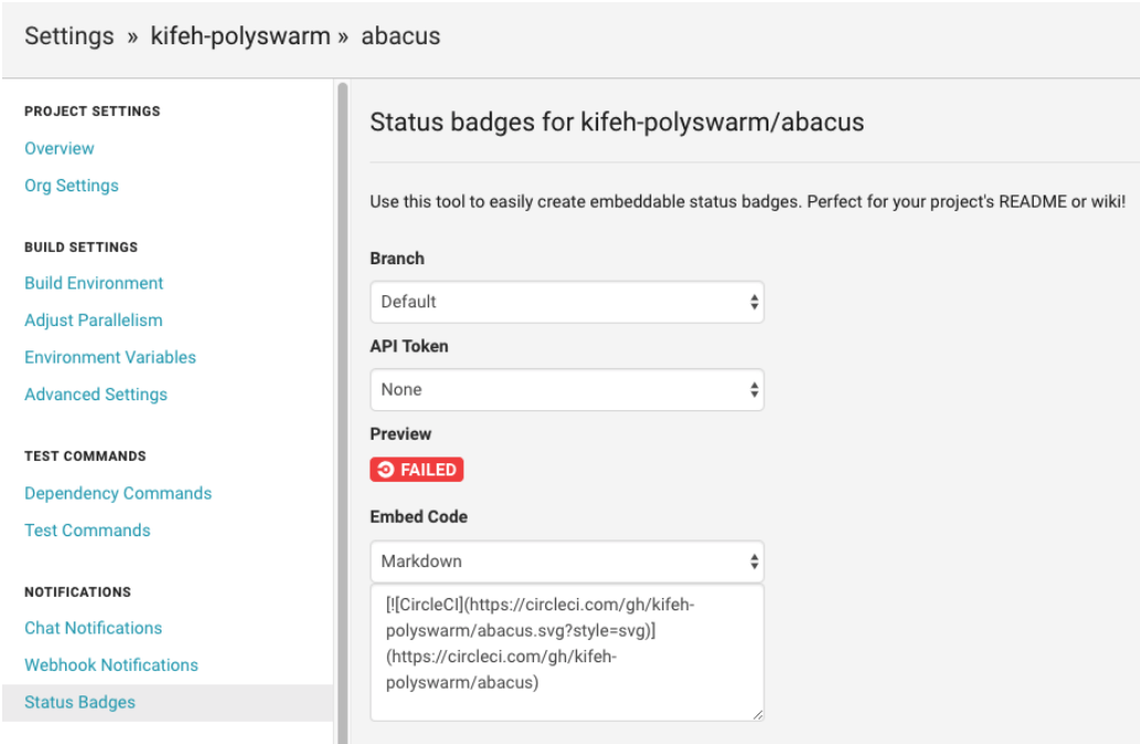
Figure 6.16: Status badges
