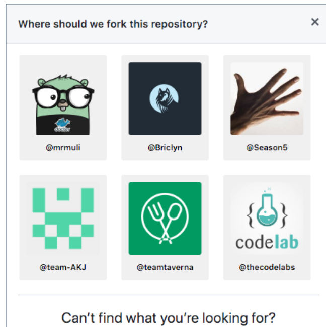
Figure 5.3: Fork location
