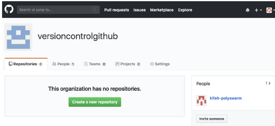
Figure 1.16: versioncontrolgithub
