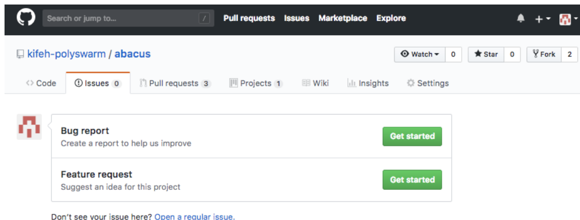
Figure 4.6: Getting started
